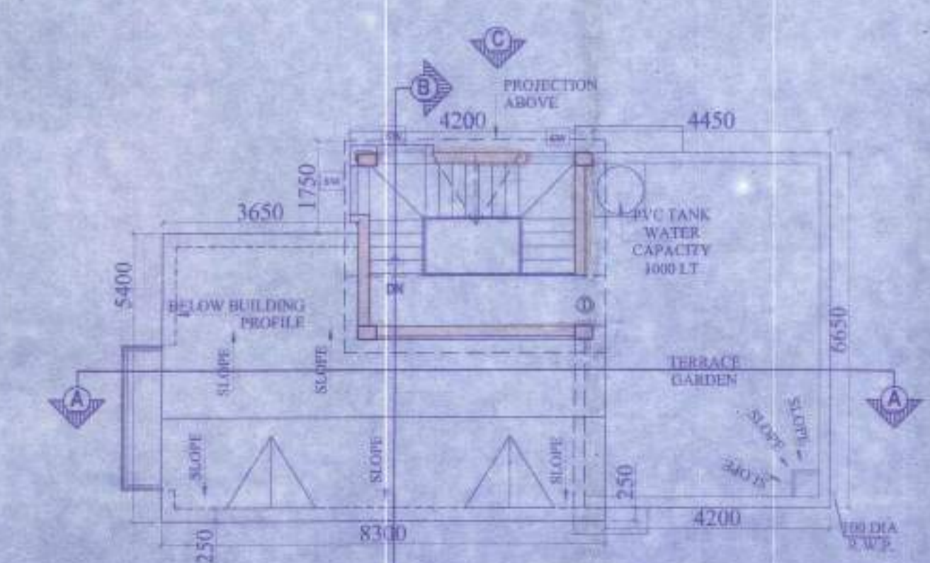
ROOF PLAN
