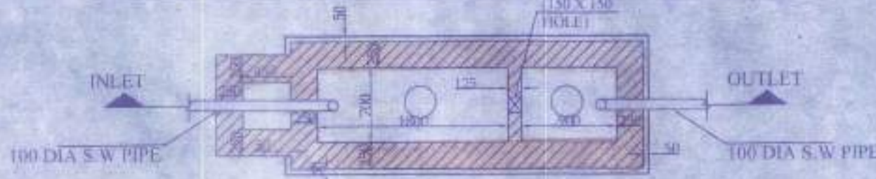
SECTION OF SEPTIC TANK
